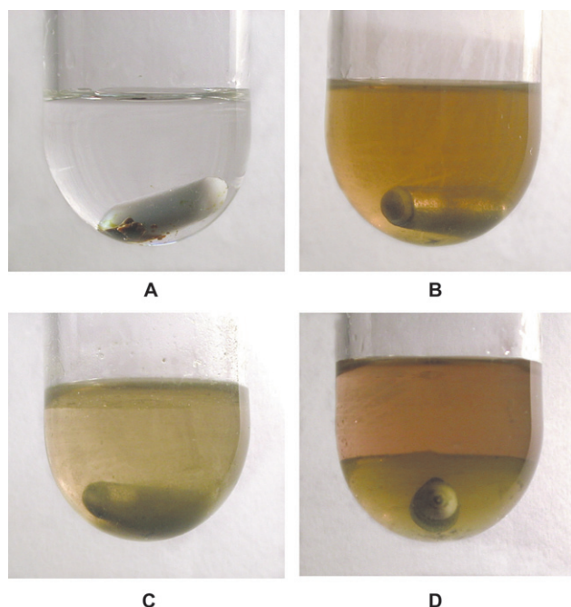
Fig. 3 Photographs of a recycling sequence analogous to the first entry in Table 3 ( 7 , methyl acrylate) but with 0.5 mol% 7 . A , before heating, with undissolved 7 ; B , after 2 h at 100 °C; C , after cooling to room temperature, with precipitated palladium complexes; D , after addition of C_8F_{17}Br . Reprinted from ref. 25 with permission from the American Chemical Society.
